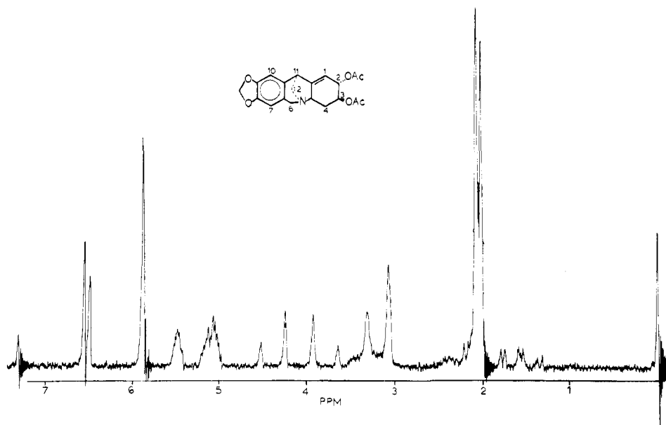
Figure 1. Nmr spectrum of O,O-diacetylpancracine.
