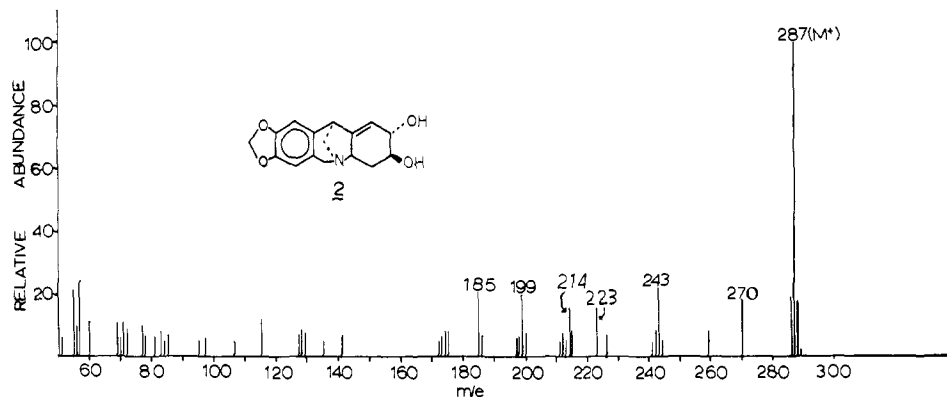
Figure 2. Mass spectrum of pancracine.
