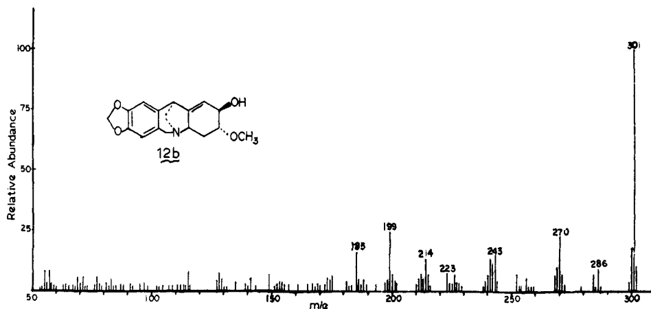
Figure 4. Mass spectrum of \alpha -isocrinamine.
