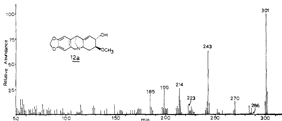
Figure 3. Mass spectrum of isohaemanthamine.
