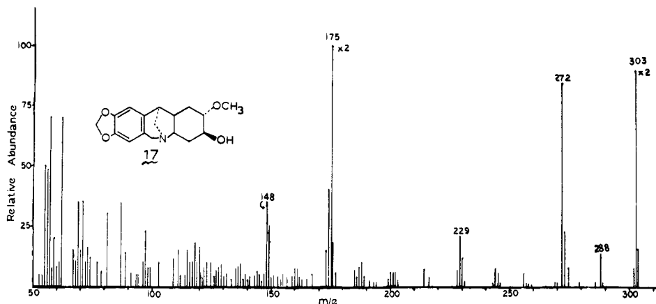
Figure 7. Mass spectrum of dihydromontanine.
