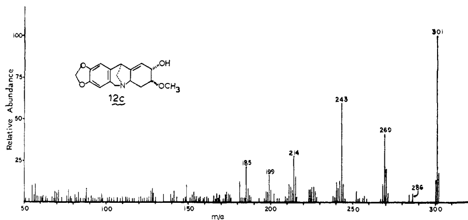
Figure 5. Mass spectrum of \beta -isocrinamine.
