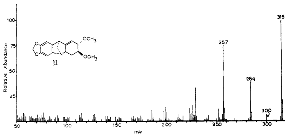
Figure 6. Mass spectrum of manthine.
